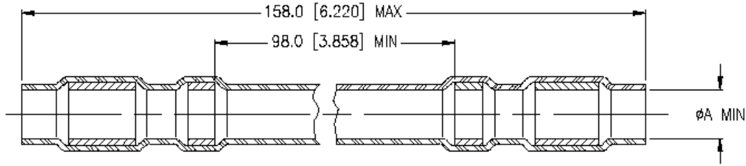
Item 1: OUTER SOLDER SLEEVE, Qty/kit: 1
