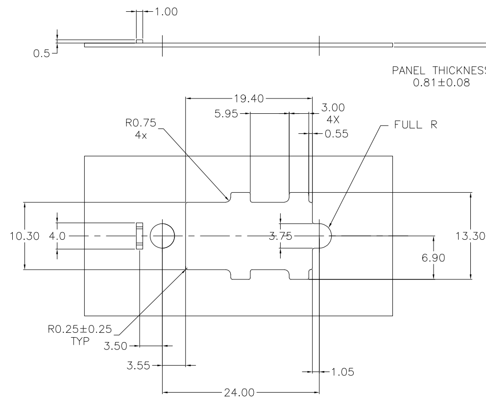
RECOMMENDED PANEL CUT-OUT (PANEL FACE SHOWN)
