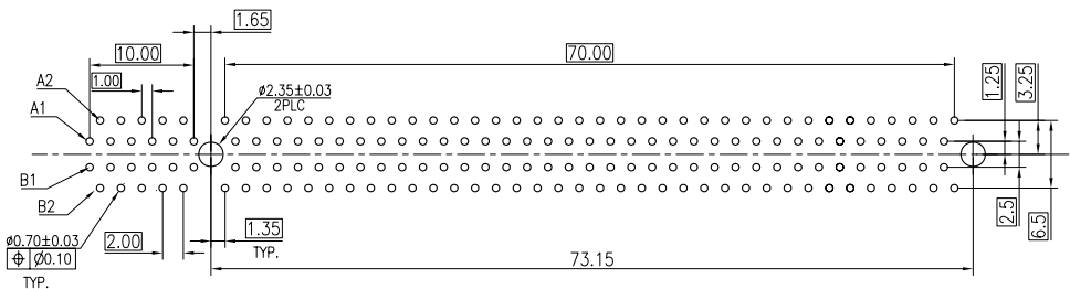
PCB LAYOUT(TOL ±0.05)
