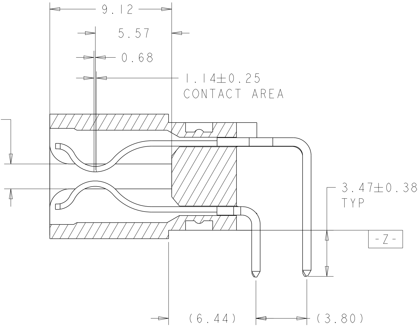
SECTION Z-Z
