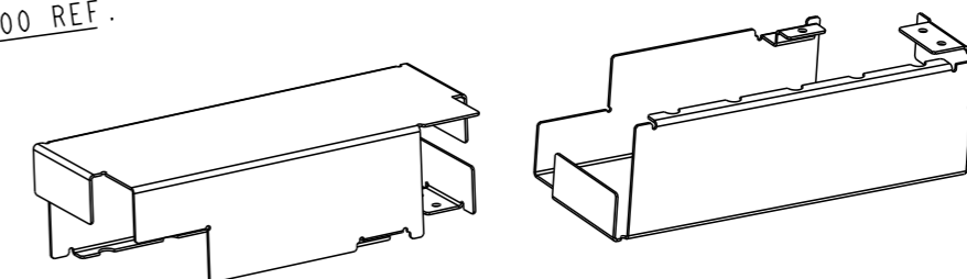
AS SHOWN P/N 2108823-1 SCALE 1:1
