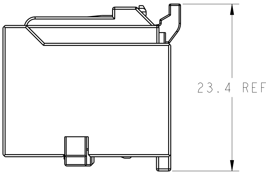
0-2295393-1 AS SHOWN WITHOUT WIRE DRESS
