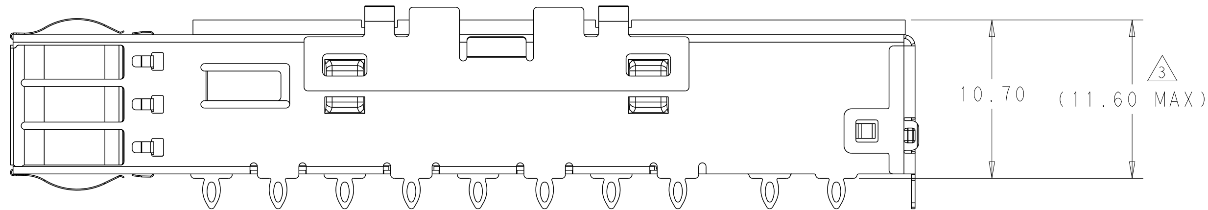
2304807-2 AS SHOWN UNSPECIFIED DIMENSIONS ARE SAME AS 2304807-1 SCALE 4:1
