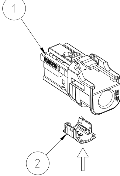
EXPLODED VIEW SCALE 2:1
