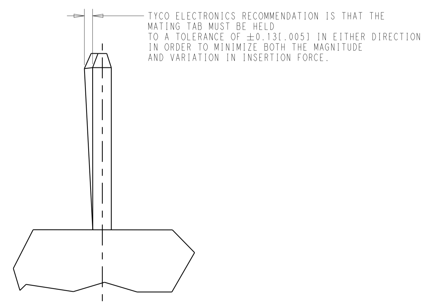
MATING TAB
