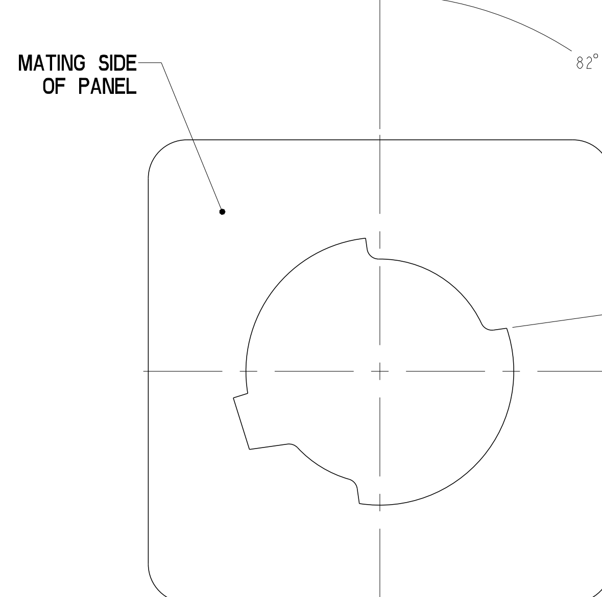
RECOMMENDED ANGLE FOR 1.47mm PANEL THICKNESS
