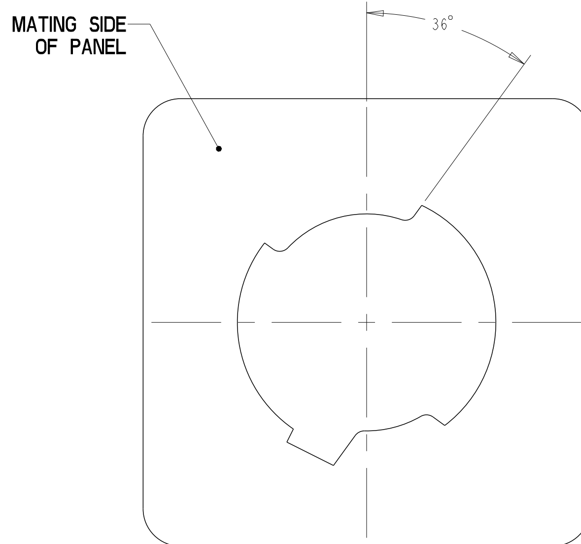
RECOMMENDED ANGLE FOR 1.47mm PANEL THICKNESS
