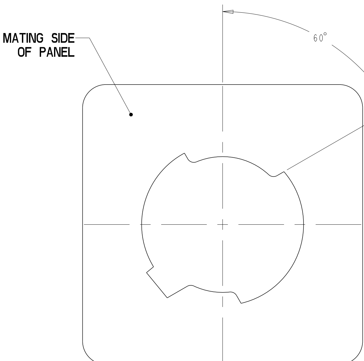
RECOMMENDED ANGLE FOR 1.27mm PANEL THICKNESS
