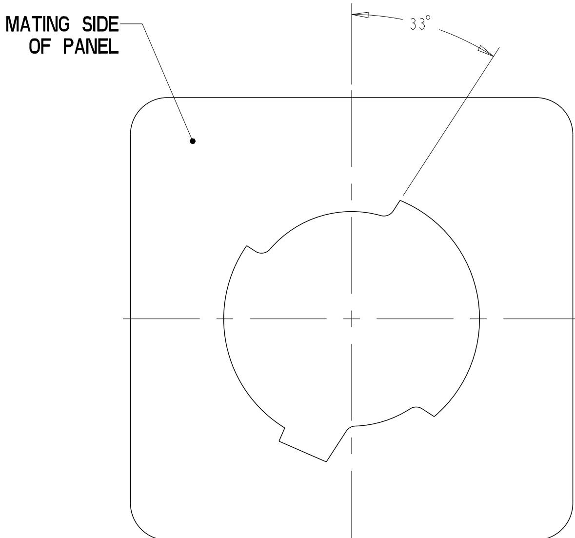
RECOMMENDED ANGLE FOR 1.27mm PANEL THICKNESS
