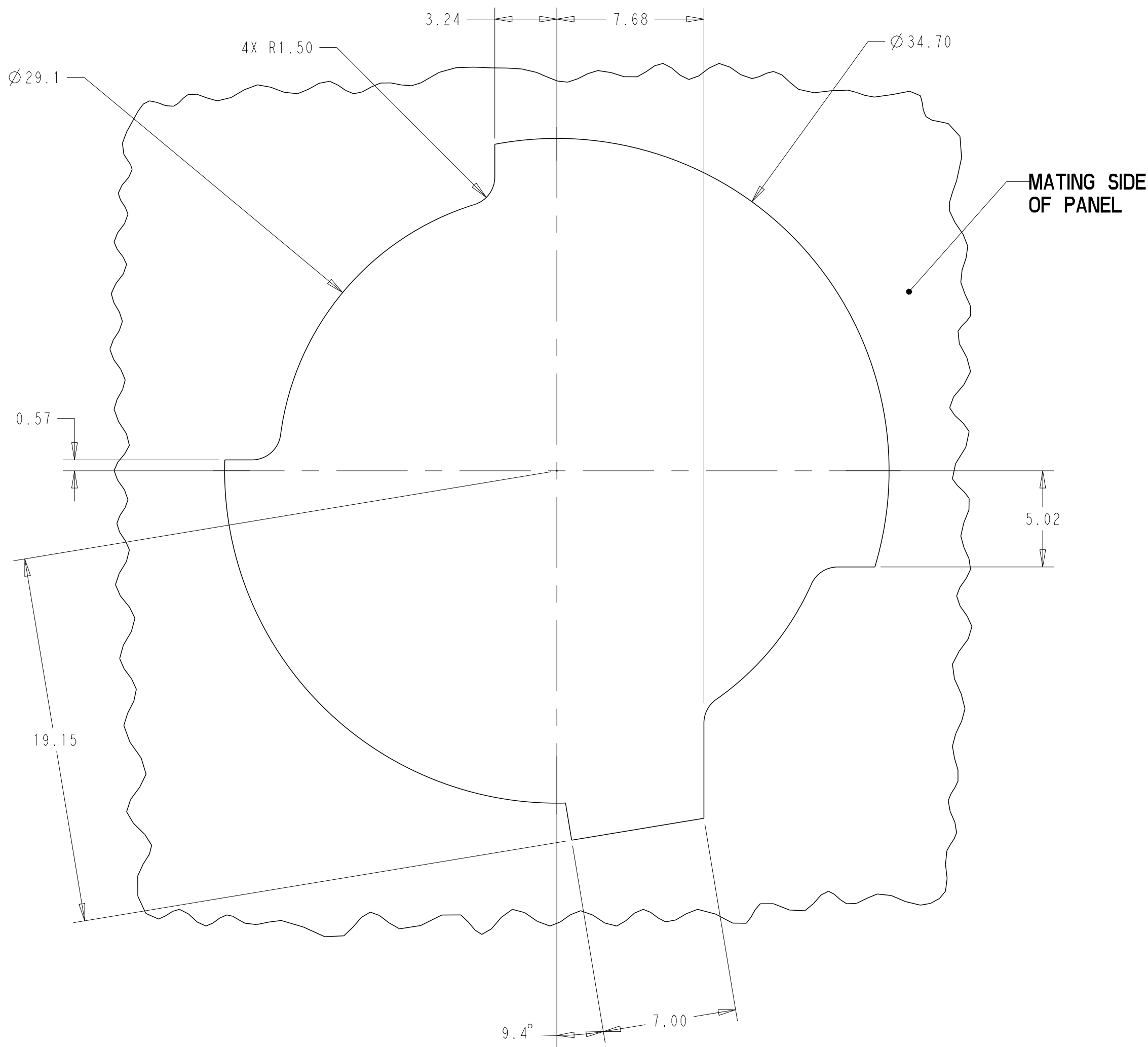
RECOMMENDED PANEL CUT-OUT (RECOMMENDED CUTOUT DIMENSION TOLERANCES \pm 0.15 ) 0.76mm PANEL THICKNESS CUTOUT SHOWN ABOVE
