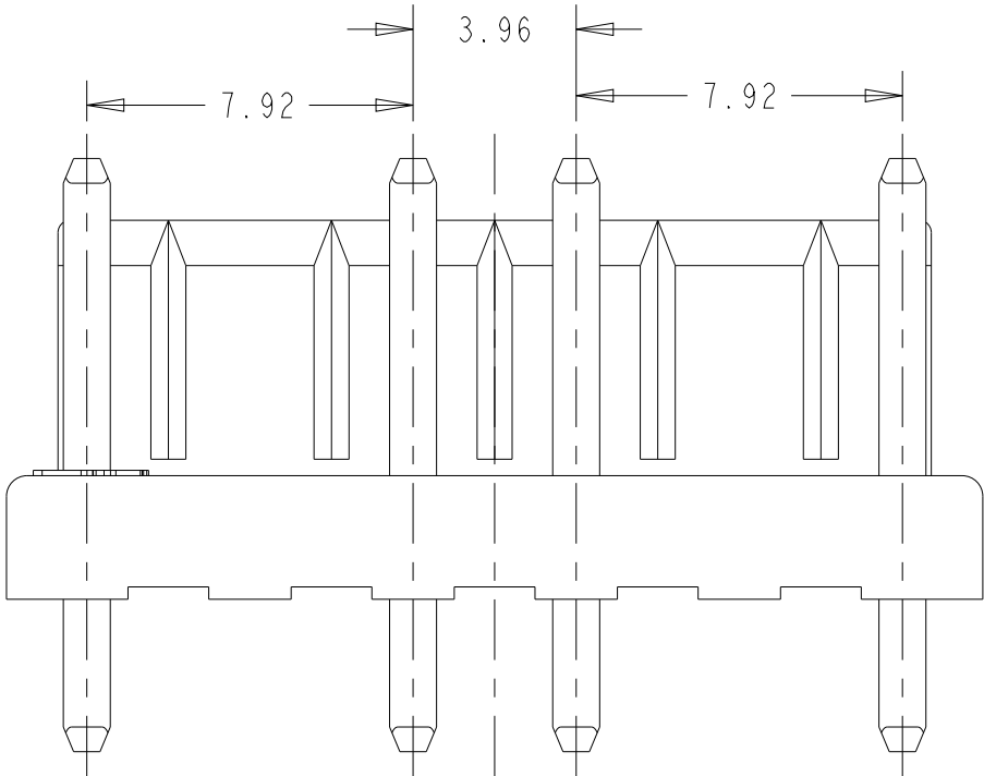
1-2375269-6 6P OMITTED 2&8
