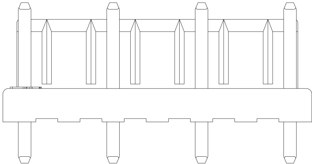
2375269-4 7P OMITTED 2,4&6
