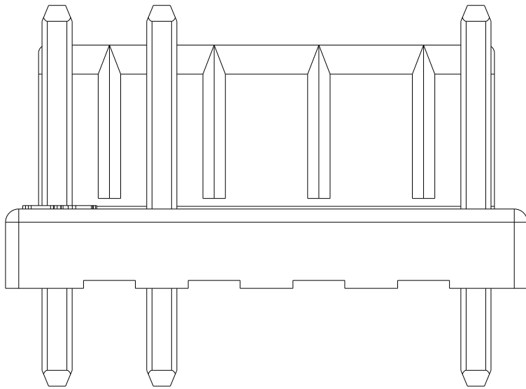
1-2375269-5 5P OMITTED 3&4
