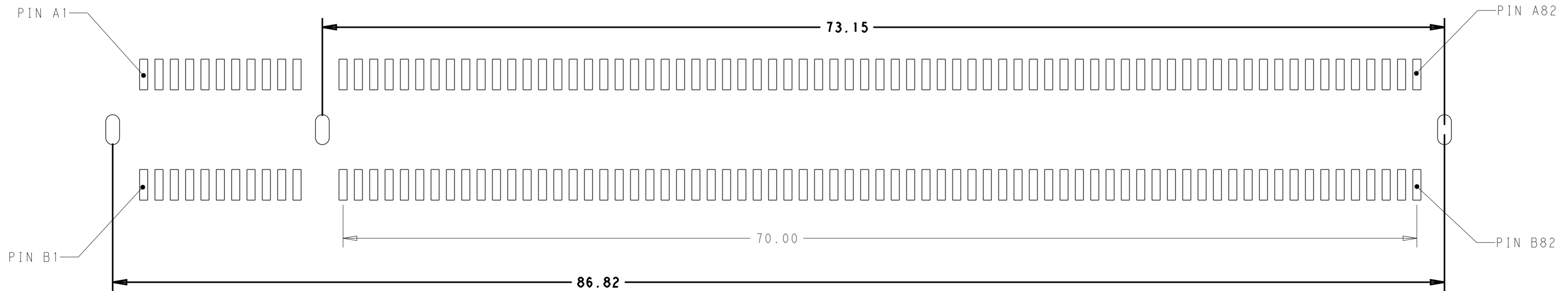
RECOMENDED PCB LAYOUT (164POS) OTHER DIMENSIONS SAME AS 36POS SCALE 5:1
