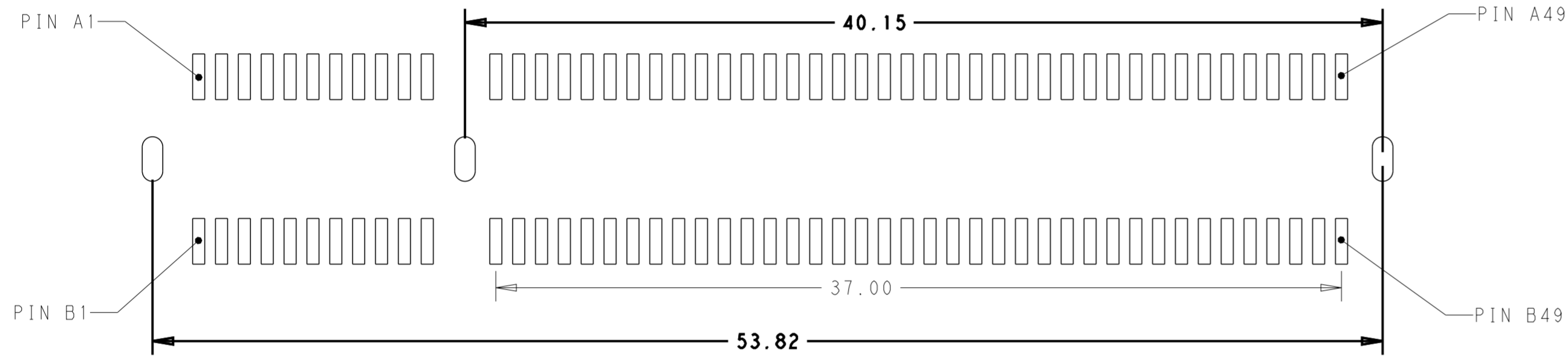
RECOMENDED PCB LAYOUT (98POS) OTHER DIMENSIONS SAME AS 36POS SCALE 5:1
