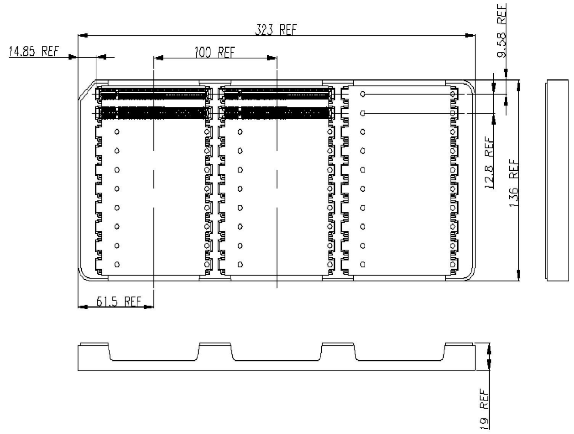
HARD TRAY: FOR 6-2399941-8/9-2399941-8/8-2399941-8 (164POS) SCALE 1:2
