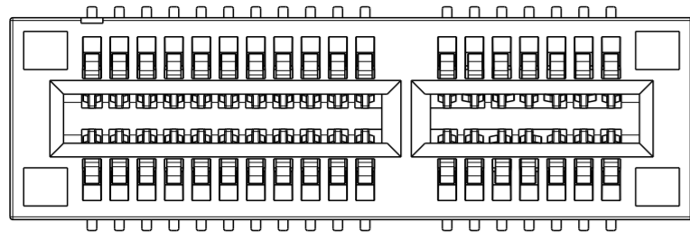
36POS AS SHOWN SCALE 4:1
