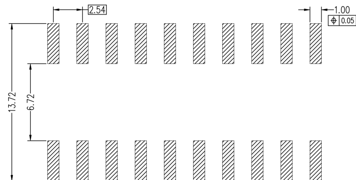
RECOMMENDED P.C.B LAYOUT (COMPONENT SIDE)(TOLERANCE:±0.05)
