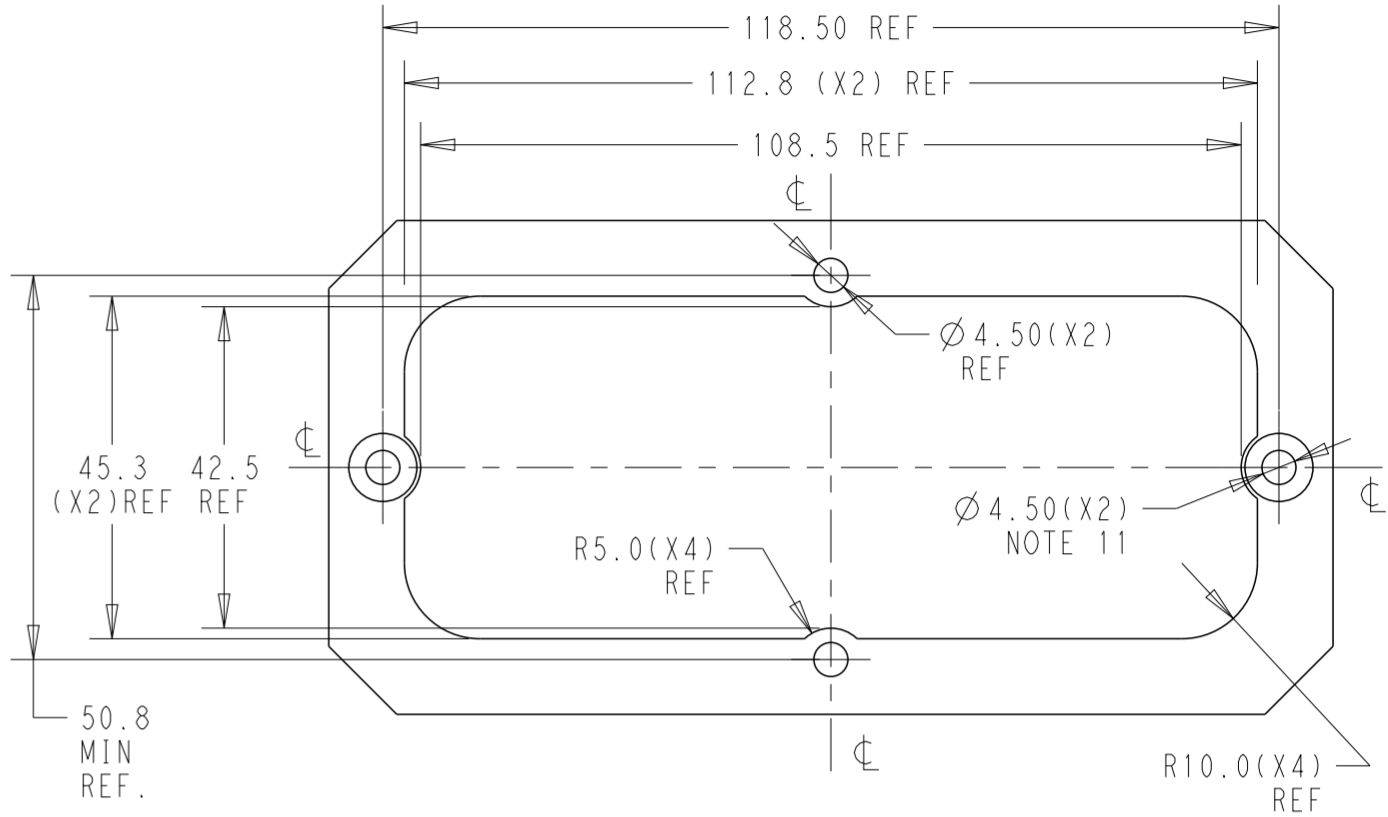
SUGGESTED VEHICLE CUT OUT (NOTE 7)
