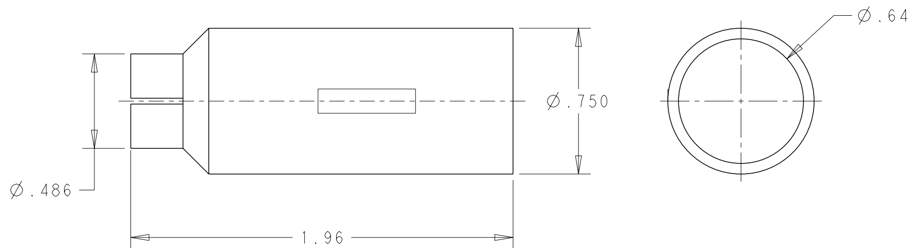
STAINLESS STEEL BOOT AND TUBING TIP (979781-000)
