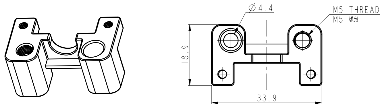
TYPE 1: MOUNTING BRACKET, COLOR ZINC PLATED 类型1: 固定架, 镀彩锌
