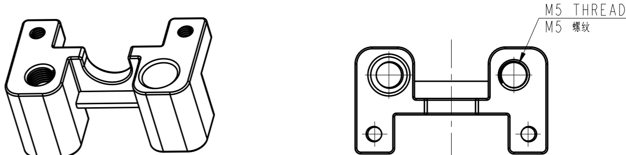
TYPE 2: MOUNTING BRACKET B, COLOR ZINC PLATED ALL DIMENSIONS ARE SAME AS TYPE 1, EXCEPT SCREW HOLES DEFINED IN THIS TYPE. 类型2: 固定架B, 镀彩锌 除了在本类型中定义的螺丝孔外, 其它尺寸同类型1.
