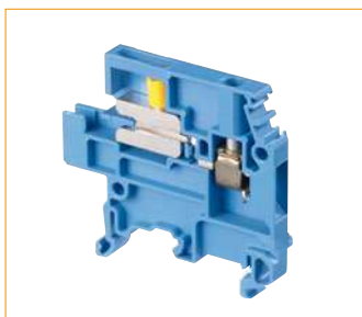
Neutral disconnect: screw clamp terminal blocks
