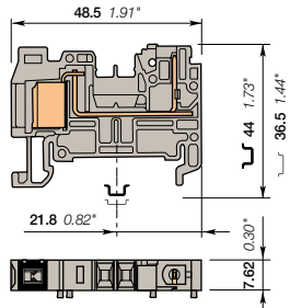
7.62 mm 0.300 in spacing
