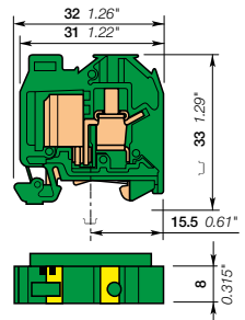
8 mm 0.315 in Spacing
