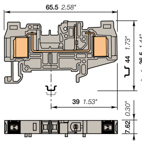
7.62 mm 0.300 in spacing
