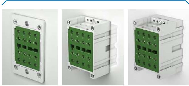
Flush mounting Half-base mounting Base mounting
