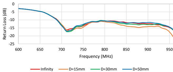
Return Loss for 2367286-1 (200mm) in Parallel Floating Metal Plate Distance (Left Side)
