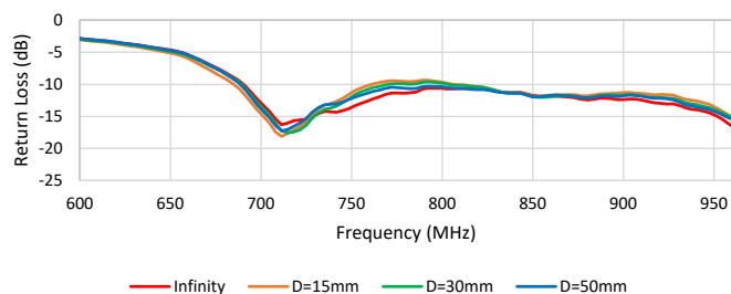
Return Loss for 2367286-1 (200mm) in Parallel Floating Metal Plate Distance (Right Side)
