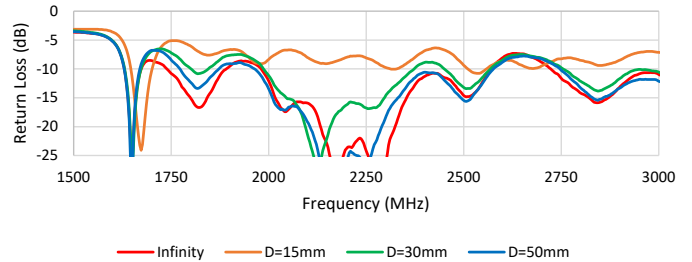
Return Loss for 2367286-1 (200mm) in Parallel Floating Metal Plate Distance (Centered)
