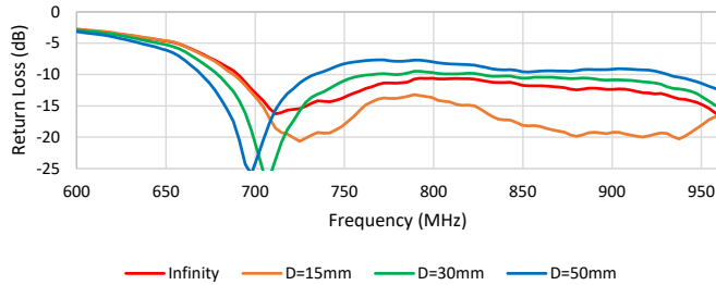
Return Loss for 2367286-1 (200mm) in Parallel Floating Metal Plate Distance (Centered)
