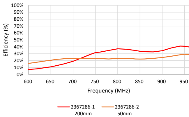
Efficiency (PN:2367286-X)
