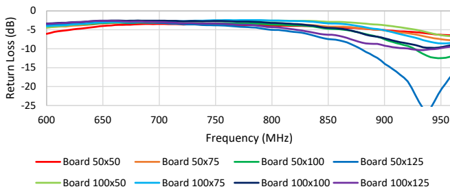
Return Loss for 2367286-2 (50mm) in Orthogonal Ground Plane Distance
