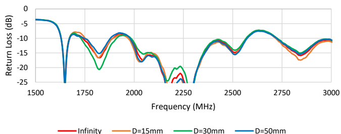
Return Loss for 2367286-1 (200mm) in Parallel Floating Metal Plate Distance (Right Side)
