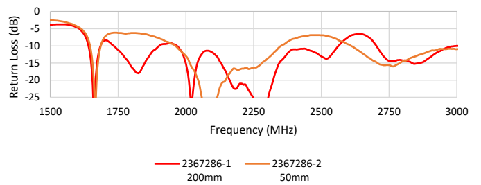
Return Loss for 2367286-X in Co-Plane Ground Plane Size (100 x 125mm)
