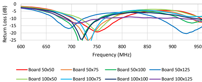
Return Loss for 2367286-1 (200mm) in Orthogonal Ground Plane Distance
