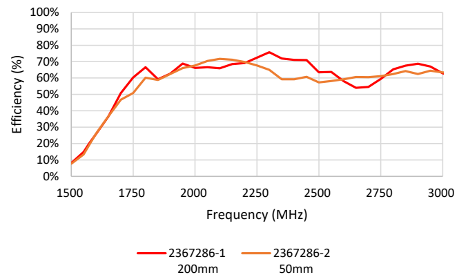
Efficiency (PN:2367286-X)
