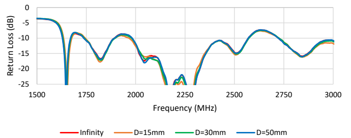
Return Loss for 2367286-1 (200mm) in Parallel Floating Metal Plate Distance (Left Side)
