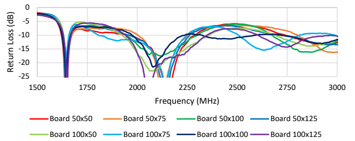
Return Loss for 2367286-2 (50mm) in Orthogonal Ground Plane Distance
