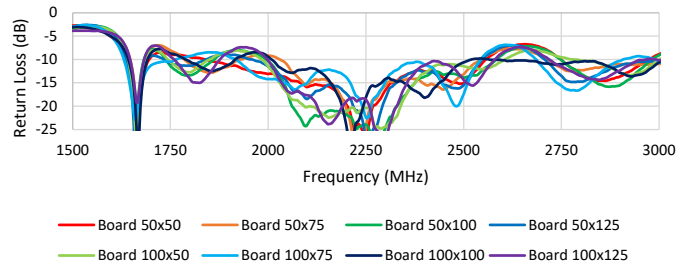
Return Loss for 2367286-1 (200mm) in Orthogonal Ground Plane Distance
