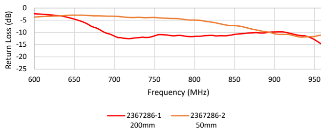
Return Loss for 2367286-X in Co-Plane Ground Plane Size (100 x 125mm)
