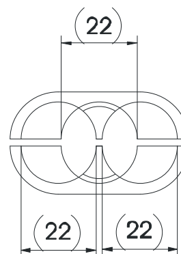
Cable entry
