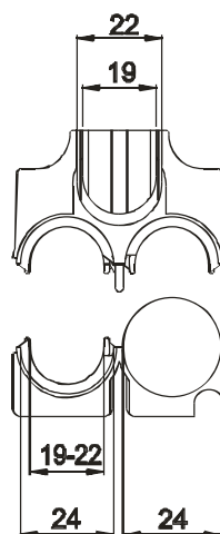
Cable entry
