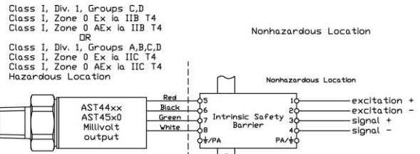
Figure 1: Wiring diagram for 4-wire, mV output
