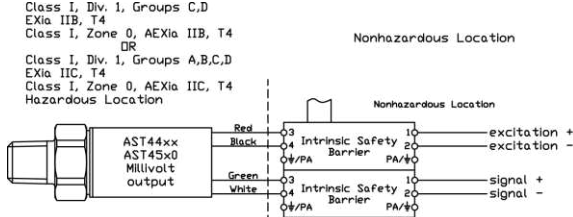
Figure 1: Wiring diagram for 4-wire, mV output
