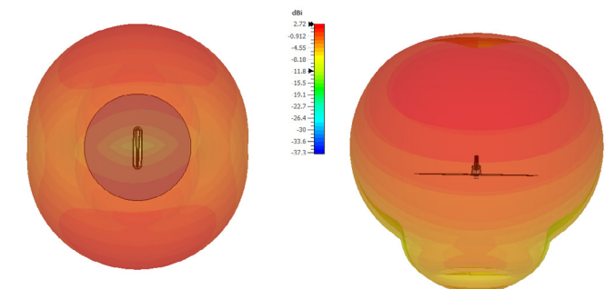
Radiation Patterns at 698 MHz
