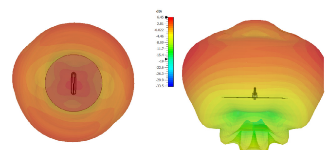
Radiation Patterns at 1690 MHz
