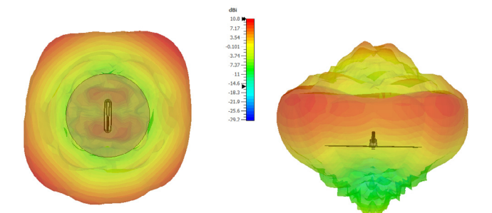
Radiation Patterns at 4900 MHz
