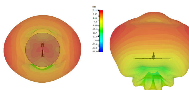
Radiation Patterns at 1500 MHz
