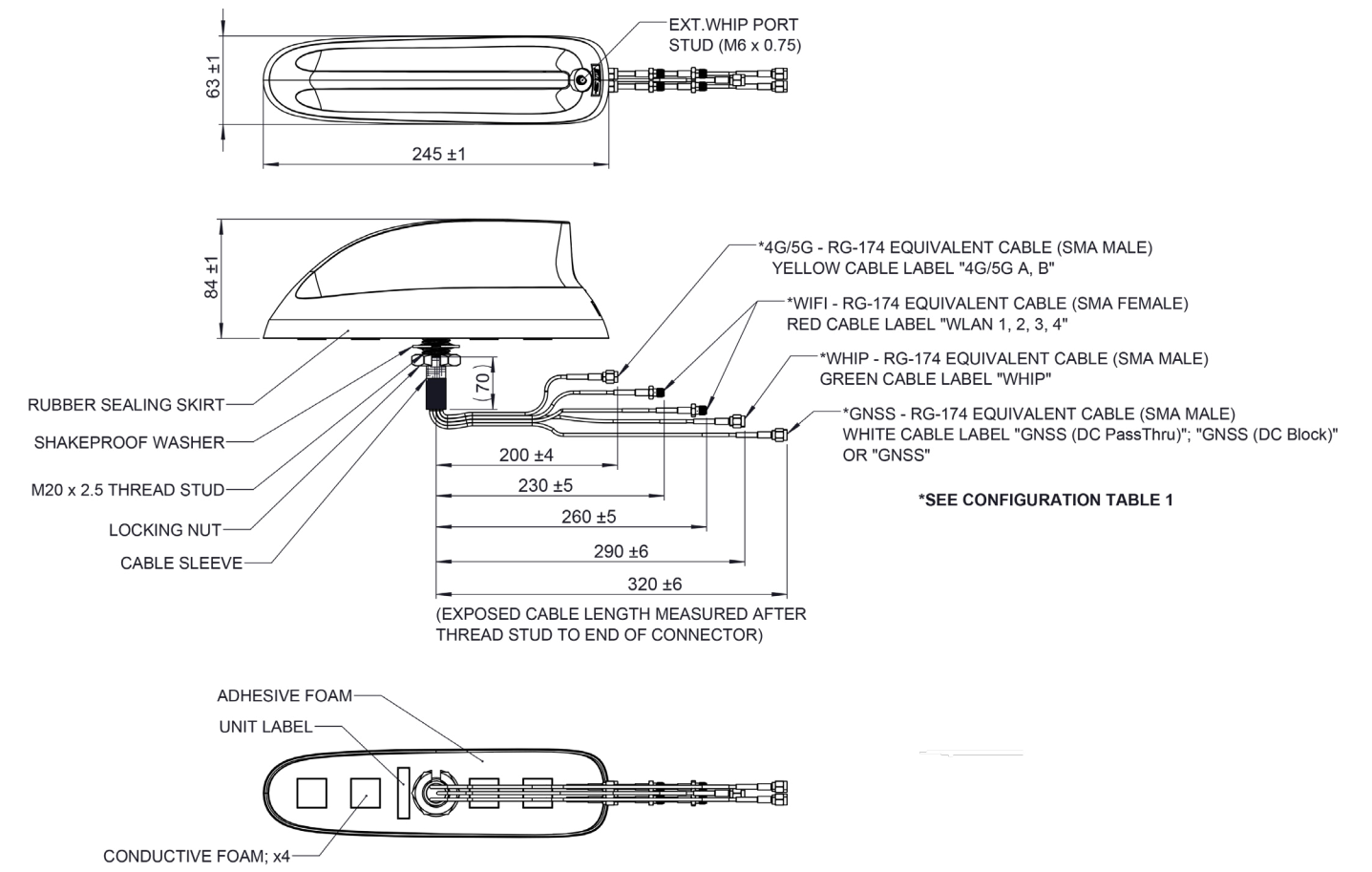
6, 7, 8 & 9 Port (Inc. Whip Models)
