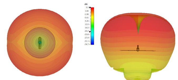
Radiation Patterns at 960 MHz
