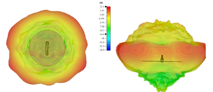
Radiation Patterns at 6000 MHz
