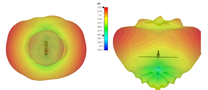
Radiation Patterns at 2450 MHz
