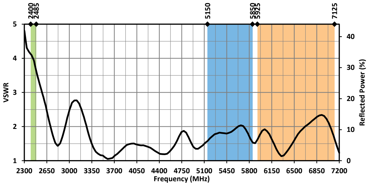
Figure 4. ANT-W63-IPW1-NP Antenna VSWR, Free Space
