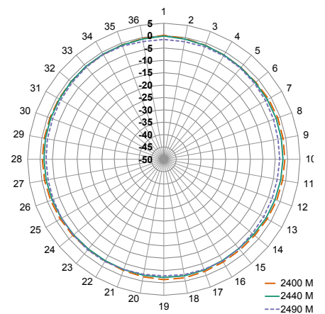
XY-Plane Gain
