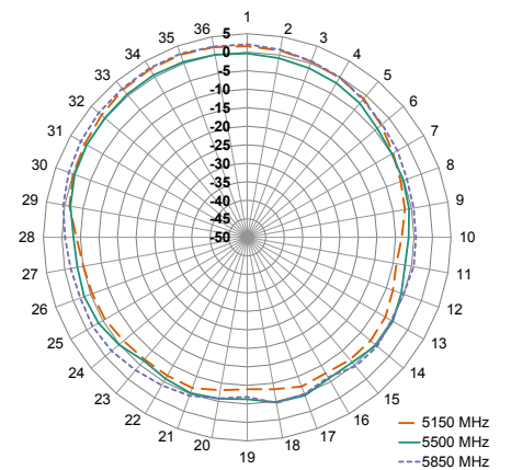
XY-Plane Gain
