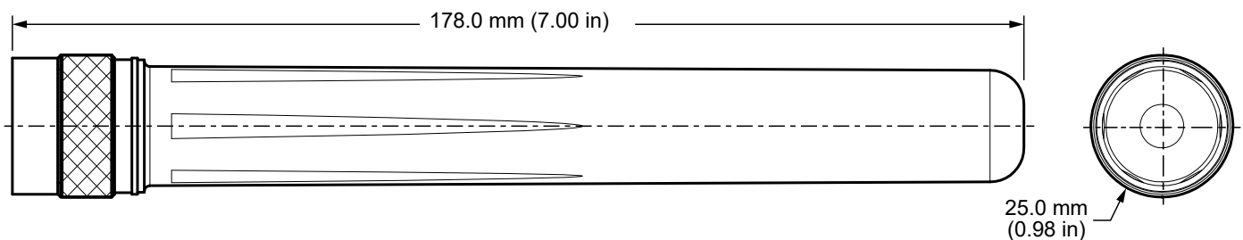
Figure 1. ANT-W63-IPW1-NP Antenna Dimensions
