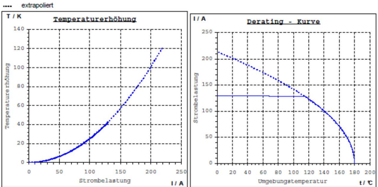
Figure1:Derating and temperature rise-1pos 25mm 2 Coroplast-Part-No.9-2611
