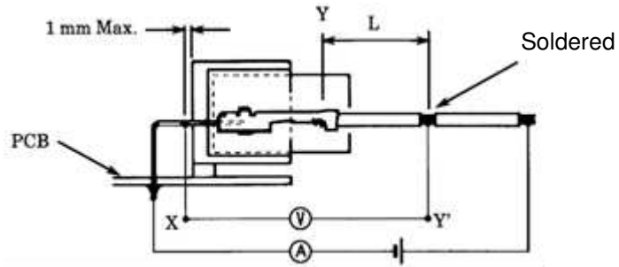
Deduct resistance of wire "L"
