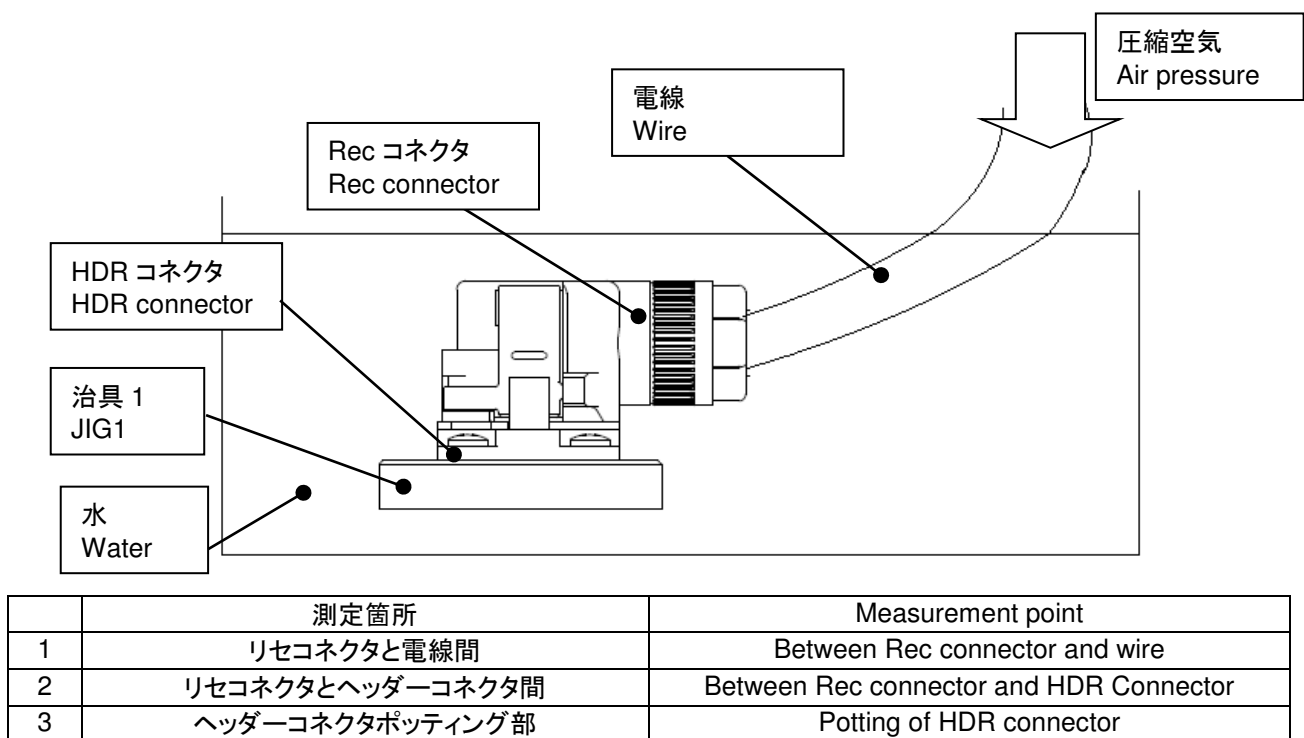
Fig.7 防水性測定 Fig.7 Waterproof Measurement
