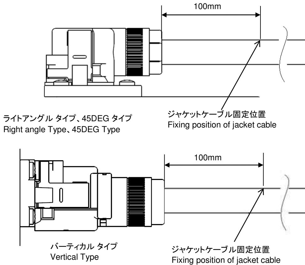
Fig.9 振動・衝撃試験固定条件 Fig.9 Fixing condition of vibration and physical shock test.
