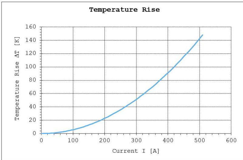
Figure 15: Temperature rise without shield current – Header 180deg 2pos +70mm² H+S-Part-No. 84100298
