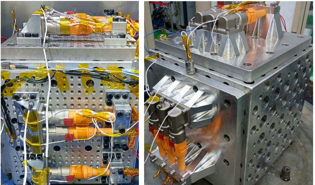
Figure 19. Vibration device
