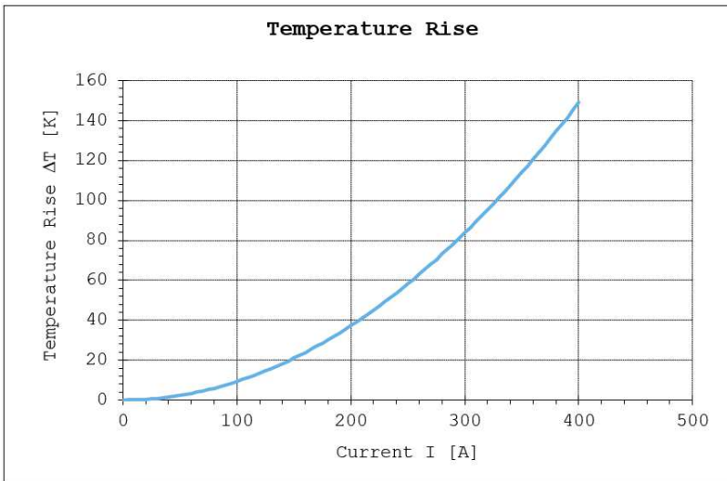
Figure 14: Temperature rise with shield current – Header 180deg 1pos +70mm² H+S-Part-No. 84100298
