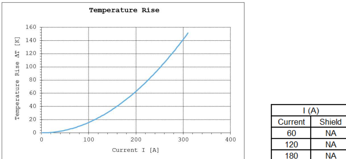
Figure 1: Temperature rise without shield current – Header 180deg 1pos +35mm 2 H+S-Part-No. 84100296
