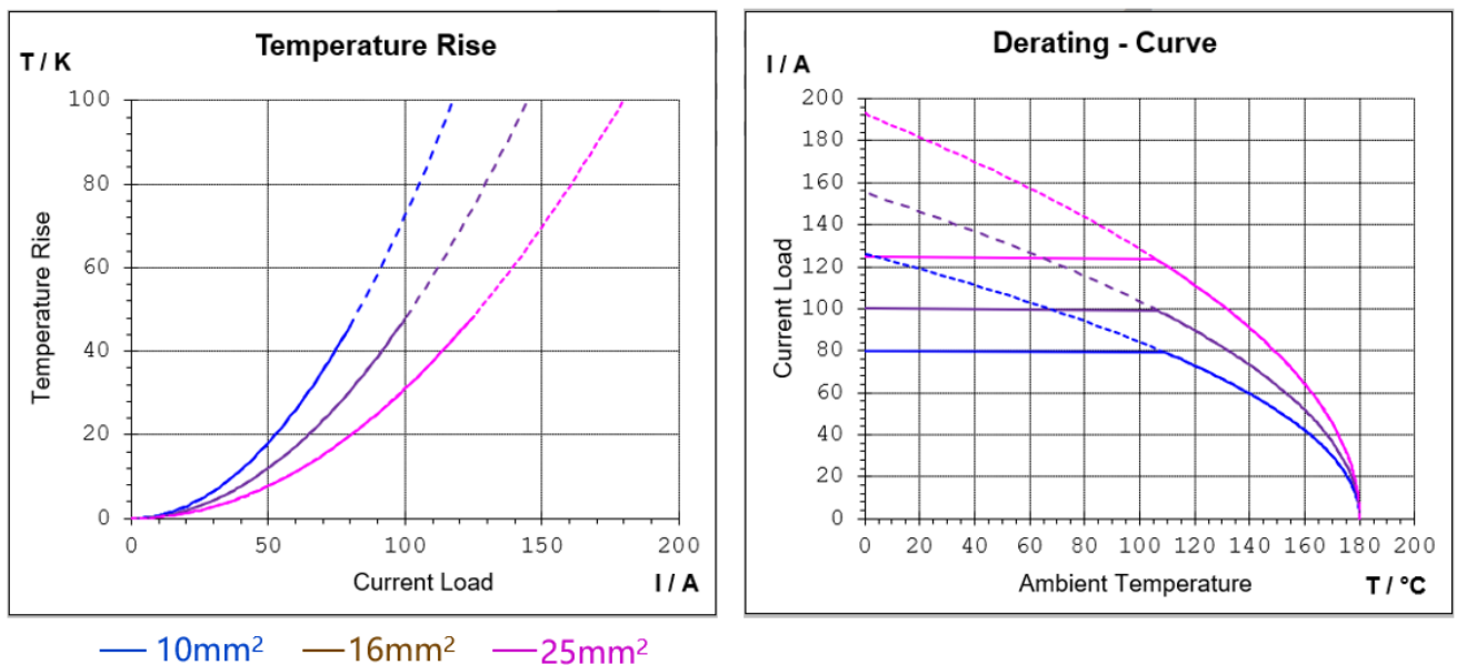
Figure1: Shield Cu cable derating and temperature rise
