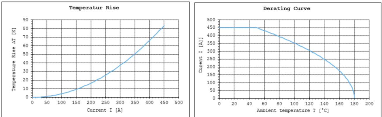
Figure 5: Derating and temperature rise – 95mm 2 Cu unshield cable
