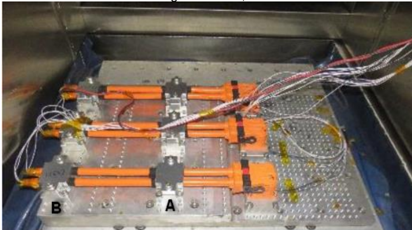
Picture 3: Vibration device (exemplary view)
