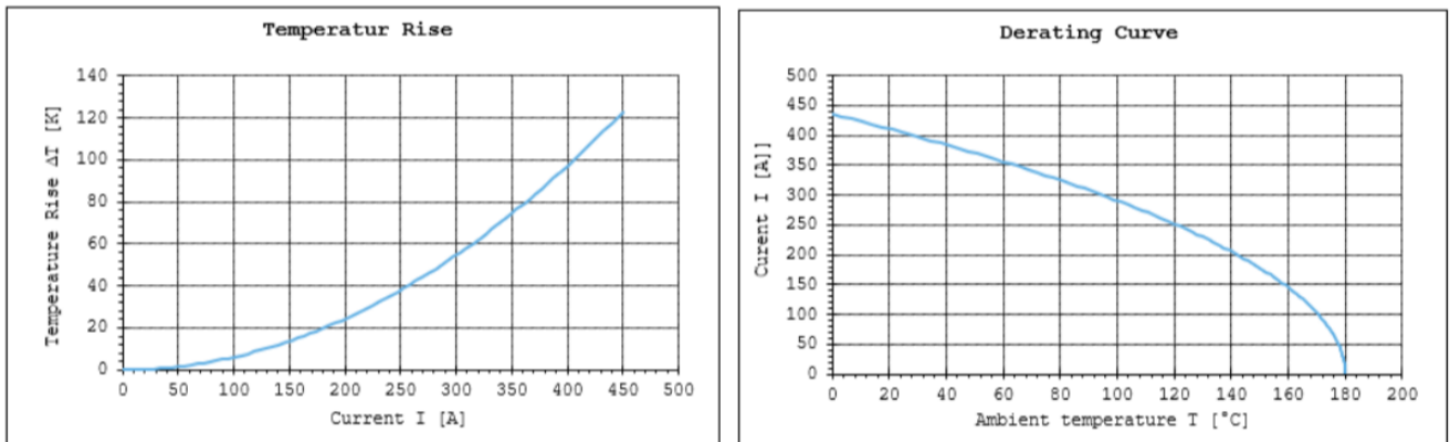
Figure 4: Derating and temperature rise – 95mm 2 Al unshield cable
