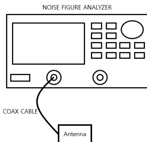
Figure 1 - VSWR Test
