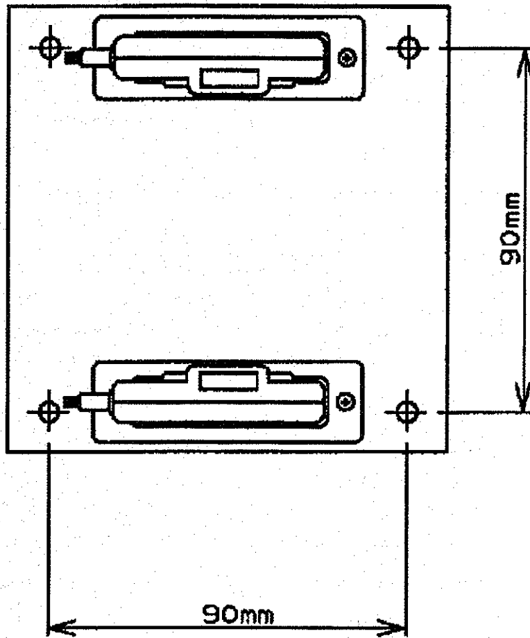
Fig. 5: Vibration Test Mounting
