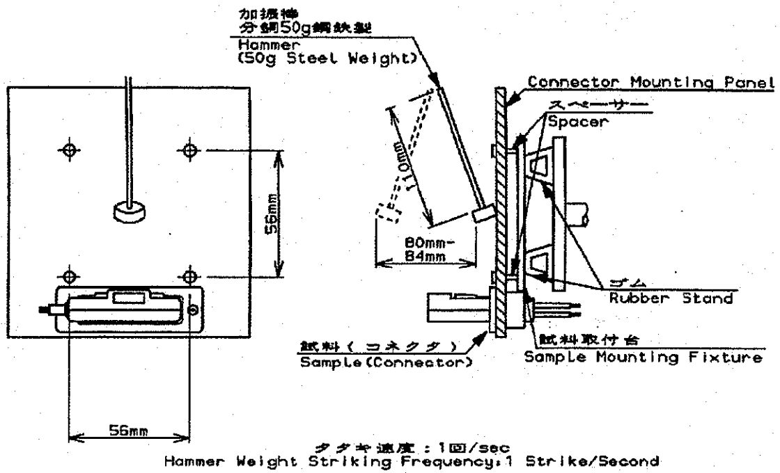
Fig. 7: Hammering Shock Test
