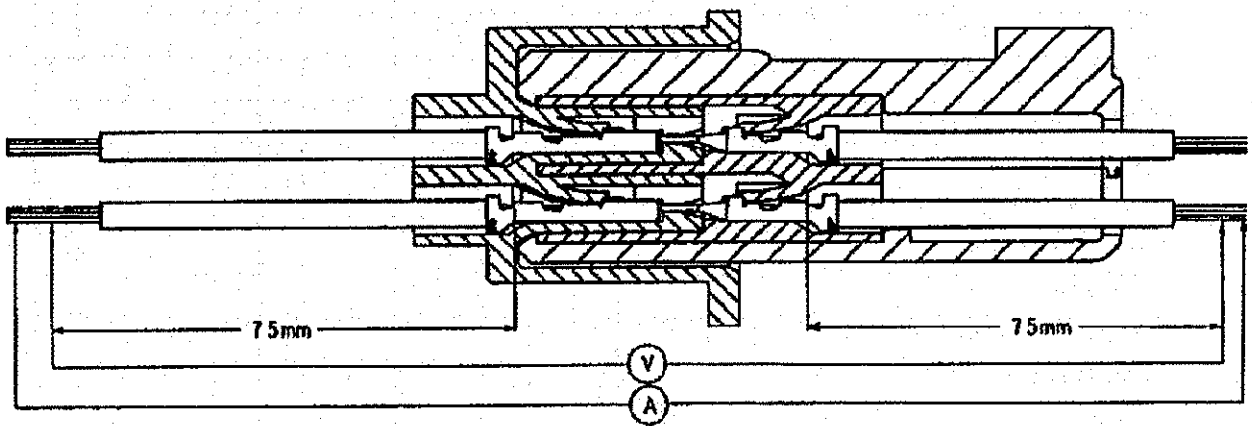
Fig 4b: (Power Line Termination Resistance Measurement Method)
