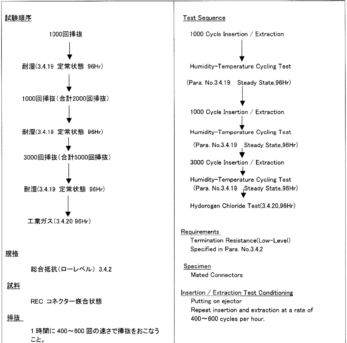
Fig.3 挿抜耐久性(オフィス外環境 5000 回) Fig.3 Durability Test (Harsh Environment)
