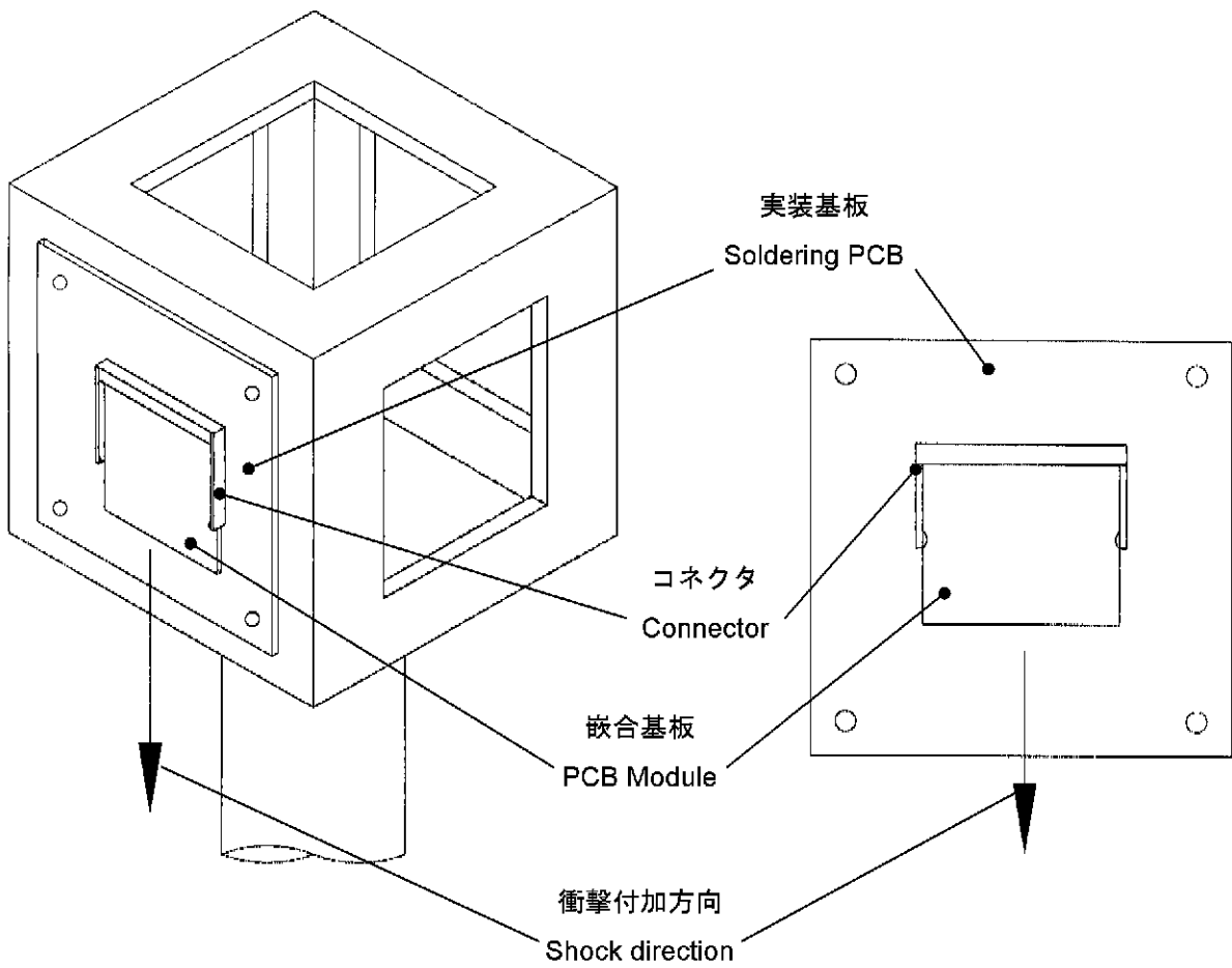
Fig. 3-2 衝撃試験 (耐久試験) Fig3-2 Physical Shock (Durable test)
