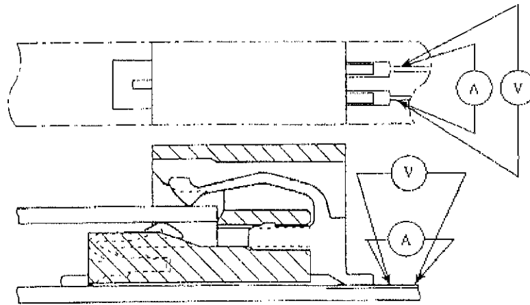
Fig. 3-1 0レベル総合抵抗測定点 Fig3-1 Termination Resistance Measuring points
