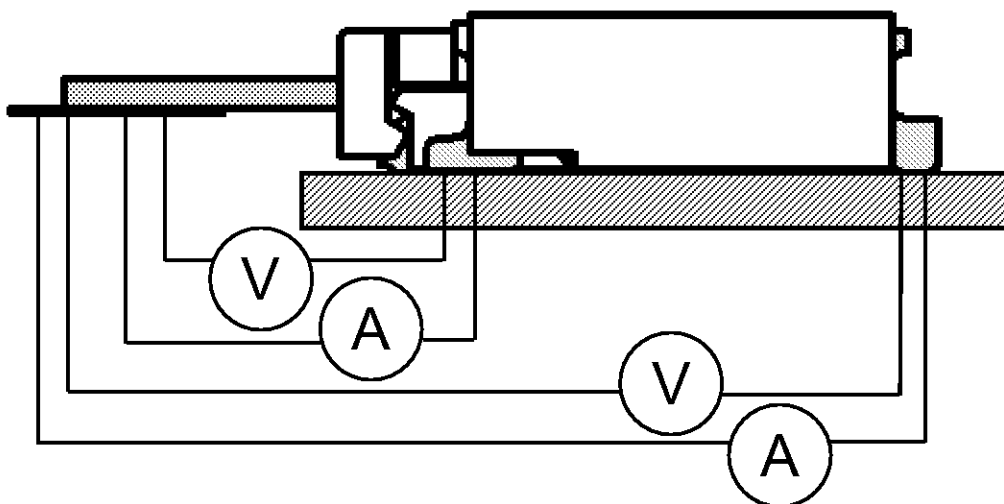
Fig.1 ローレベル総合抵抗測定 Fig.1 Low-Level Termination Resistance Measurement
