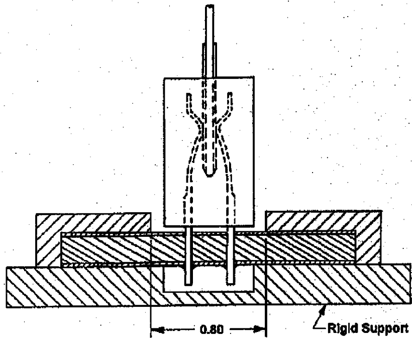
Figure 3 Vibration Mounting Fixture
