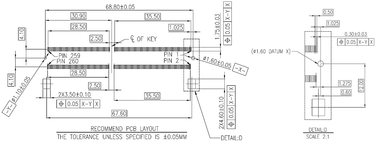
Figure 2 Recommended PCB Layout
