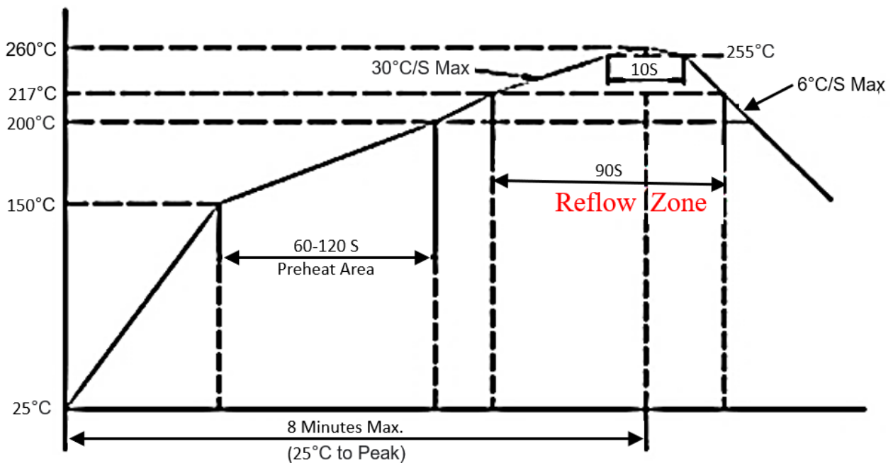
Figure 4 Recommended Reflow profile
