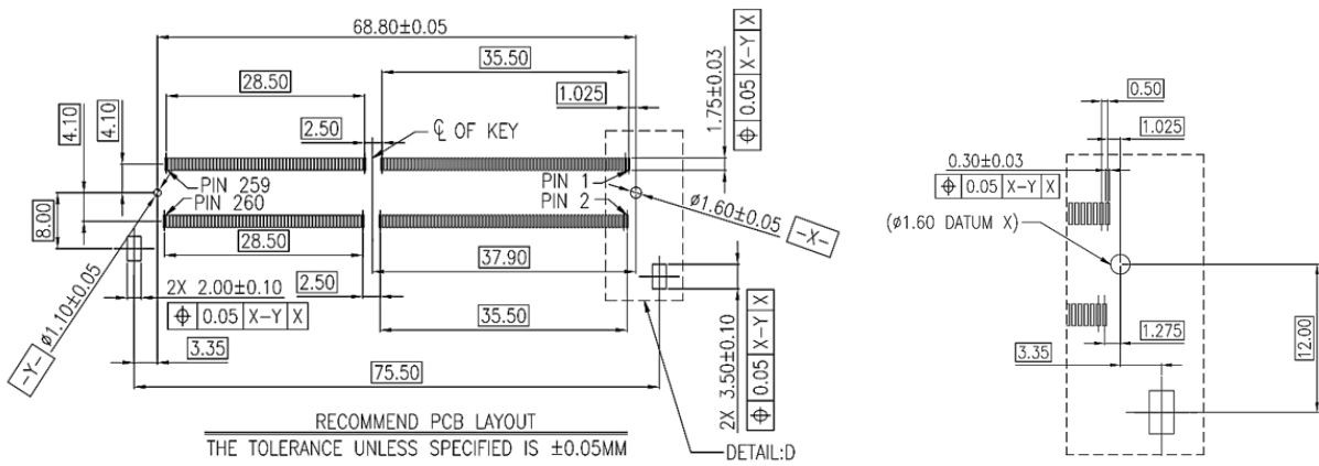
Figure 3 Recommended PCB Layout
