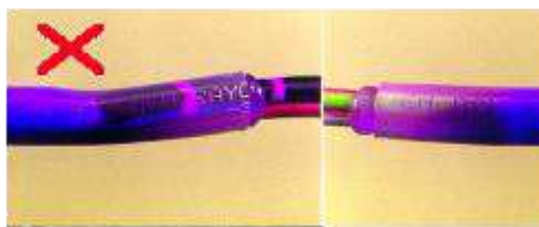
2. Overheat of tubing
