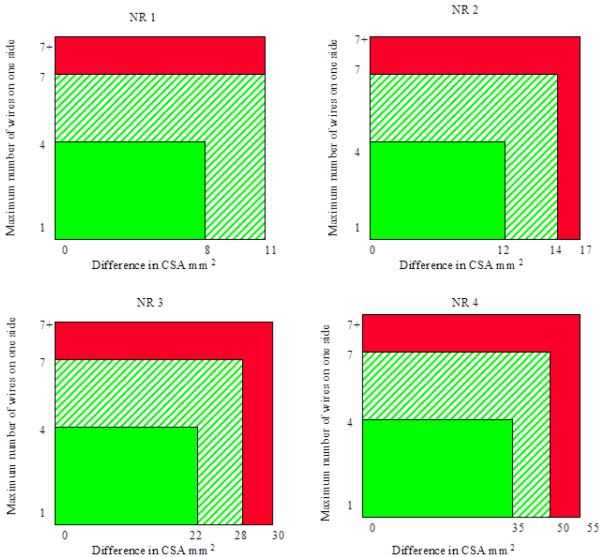
RBK-VWS-125-X Splice Matrix
