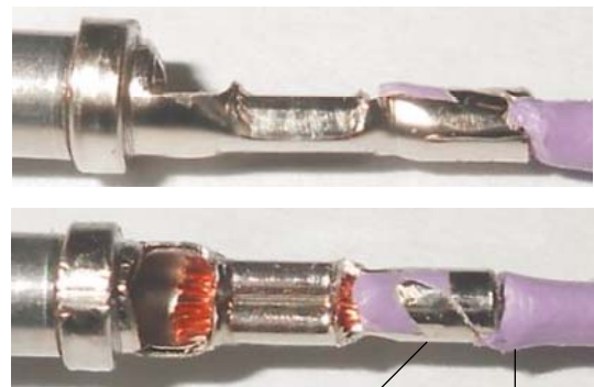
Skewing of Wire Insulation Acceptable Slight Deformation of Wire Insulation Acceptable
