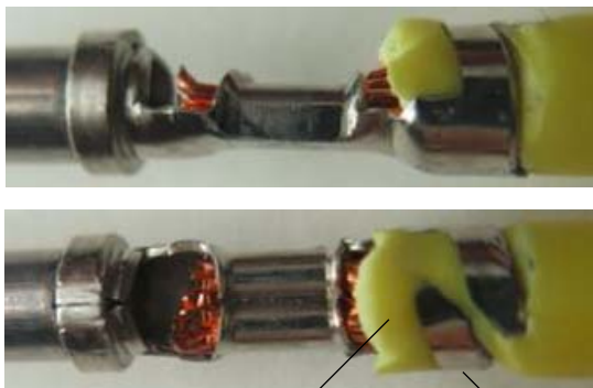
Slight Deformation of Wire Insulation Acceptable Skewing of Wire Insulation Acceptable
