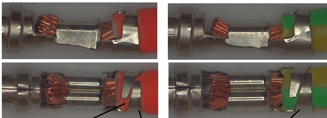
Wire Size AWG 10 SXL - Thick Shown
