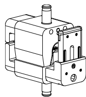
Crimping Die Assemblies and Supports for COPALUM Lite Sealed Terminals and Splices (See Table) (408-32087)
