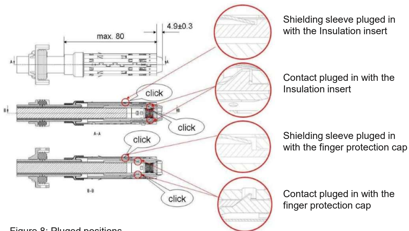
Figure 8: Plugged positions
