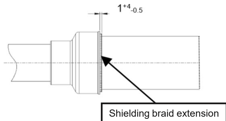
Figure 11: Braid extension
