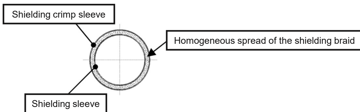
Figure 12: Braid spread
