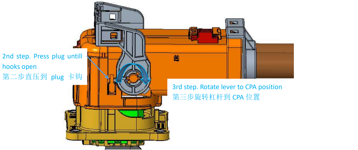
Figure 20: Rotate lever
