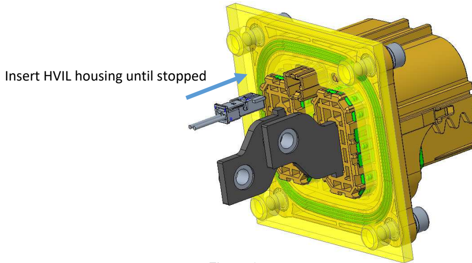
Figure 17: Insert HVIL housing
