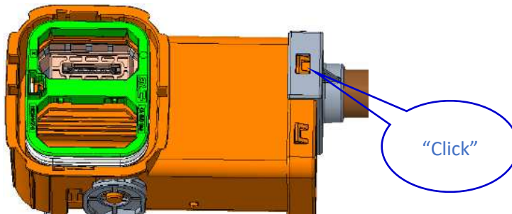
Figure 15: Assemble cable seal assy
