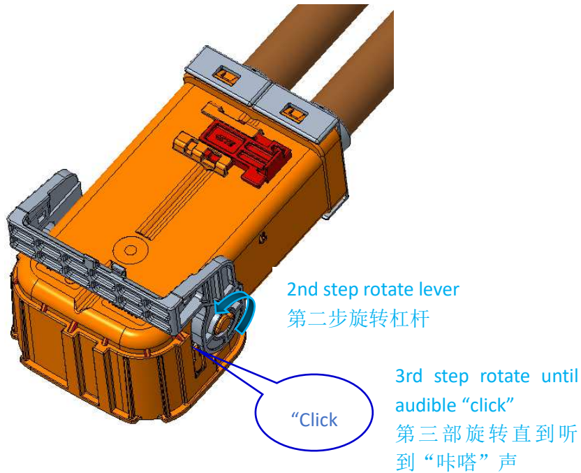
Figure 18: rotate into plug position
