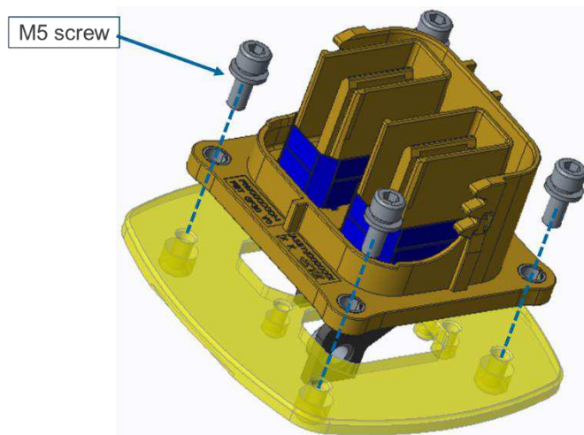
Figure 17: Assemble header to the panel
