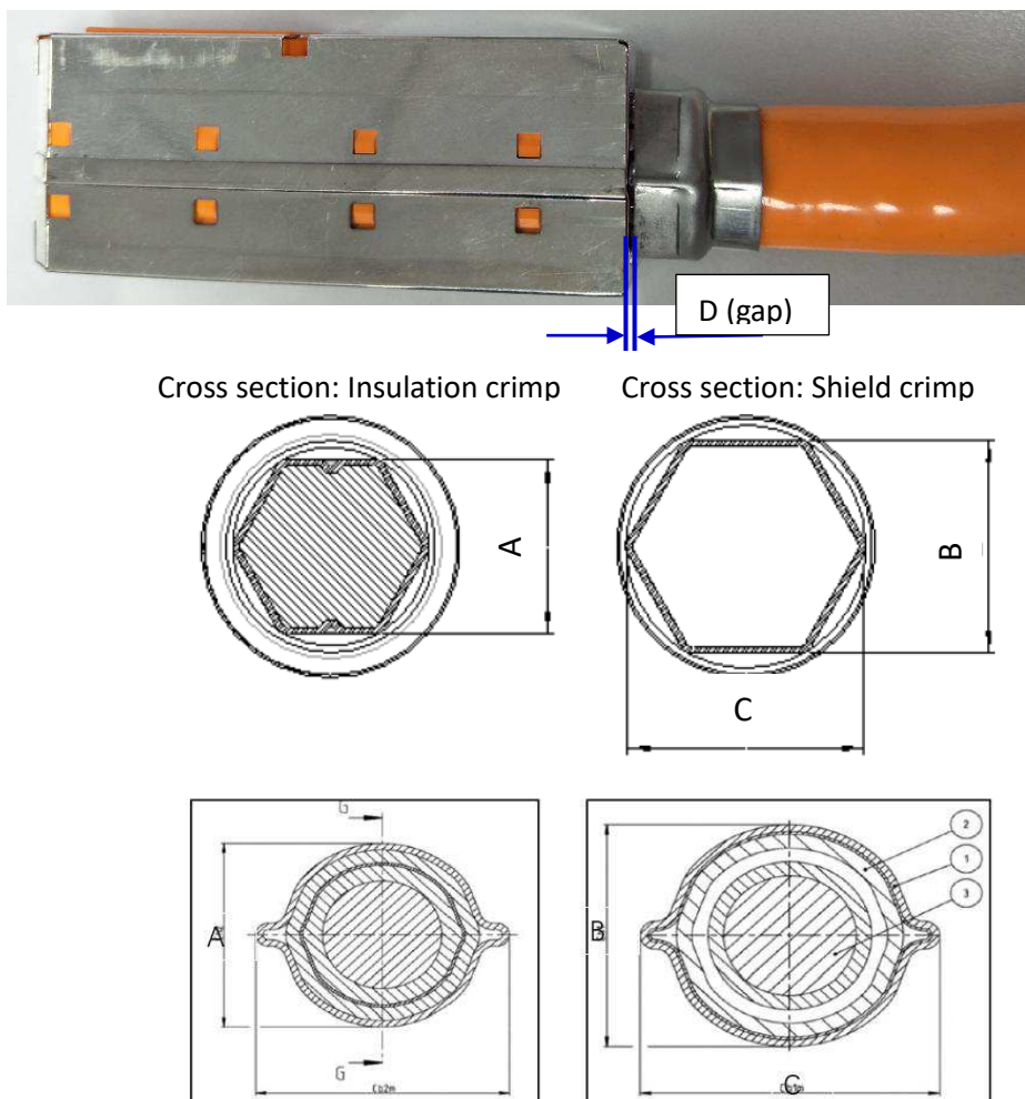
Figure 12: Crimped shield crimp ferrule
