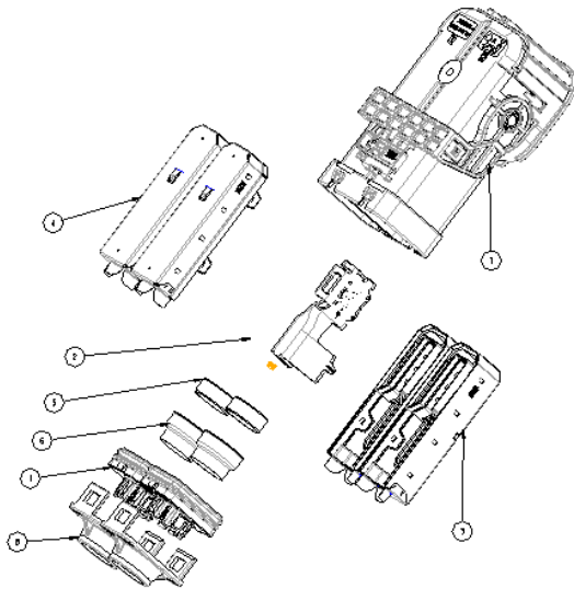
Figure2: PCON21 contact 90deg overview(shielding)
