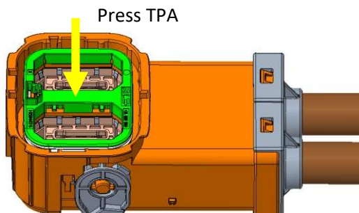
Figure 16: Press TPA
