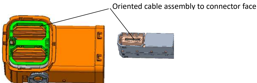
Figure 13: Oriented cable assembly to housing
