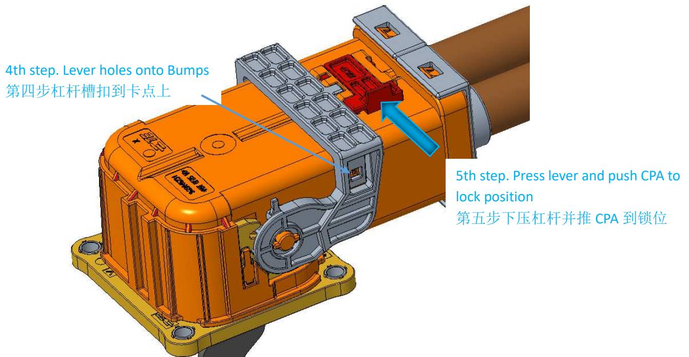
Figure 20: Lock CPA
