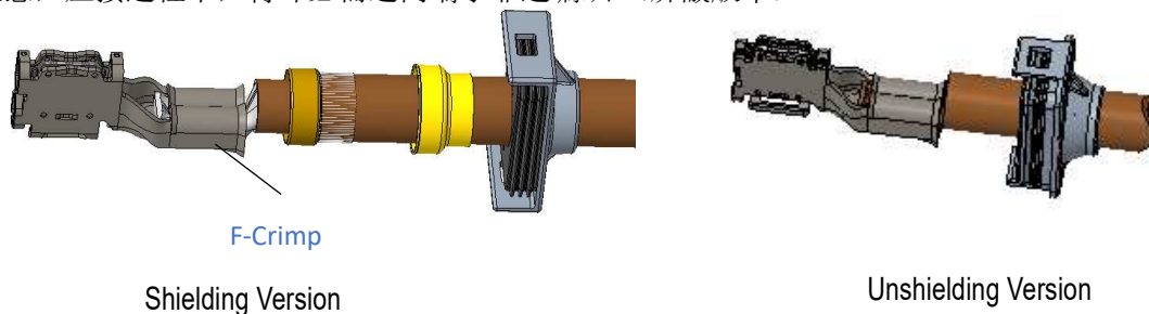
Figure 6: Contact crimp
