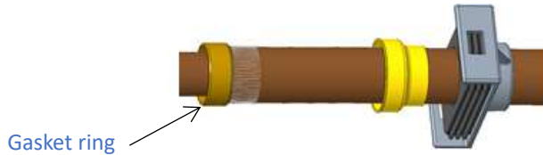
Figure 5: Comb out screening braid and assemble gasket ring
