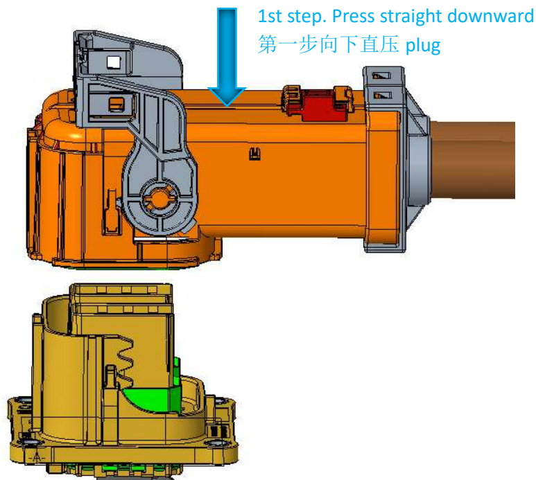
Figure 19: press plug downward
