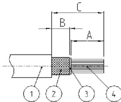
Figure 4: Cutting cable to length
