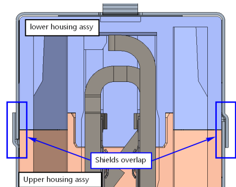
Figure 9: Shields overlap
