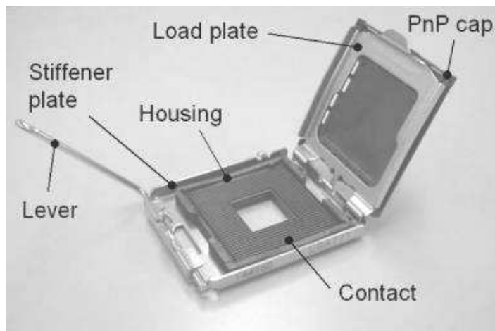
Socket configuration ( at open )
