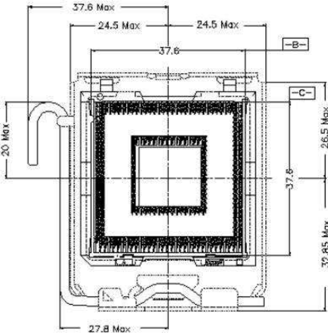
Assembly occupation area
