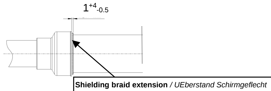
Figure 13: Braid Extension/Litzenueberstand
