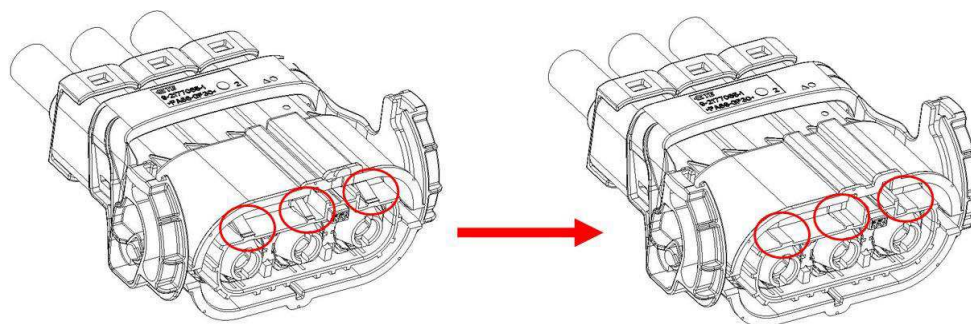
Figure 19: 3pos, End-position of seal retainer/ Dichtungshalter-Endposition
