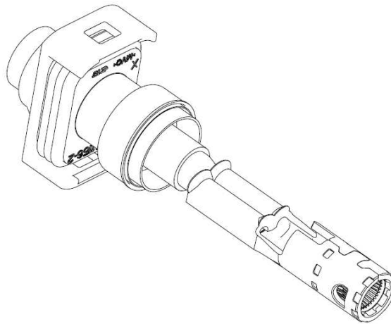
Figure 7: Contact crimp/Kontaktcrimp
