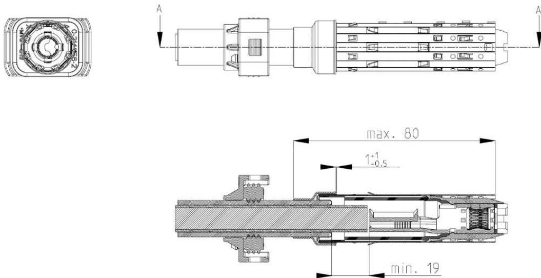
Figure 11: Cable assembly/Kabelbaugruppe
