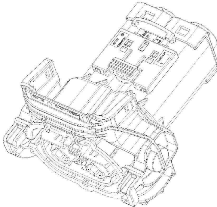
Figure 23: Open the lever by released CPA and pressed latch of CPA-Adapter.
