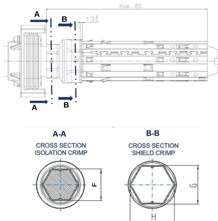
Figure 12: Inspection dimensions/Prüfmass
