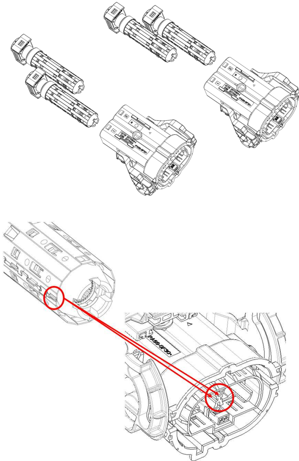
Figure 16: Assembly 2pos. connector/Montage 2-pol. Stecker
