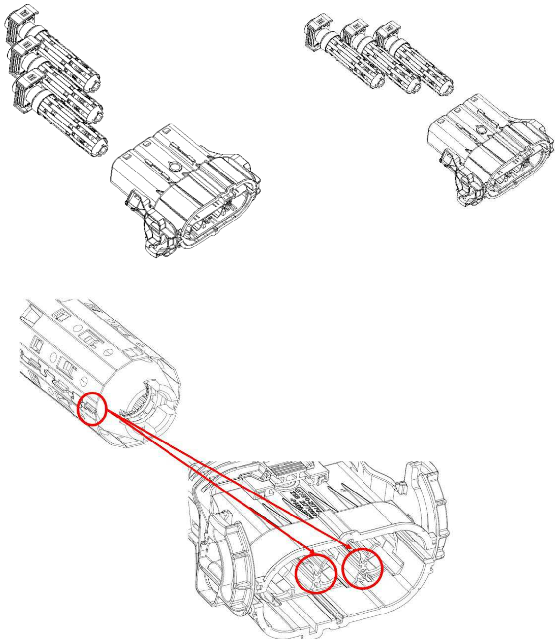
Figure 15: Assembly 3 pos. connector/Montage 3-pol. Stecker
