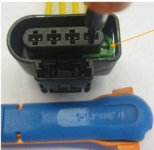
Figure 3: Contact extraction: take small screw driver for retainer shifting
