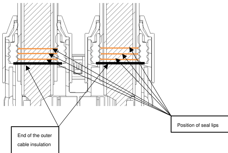
Figure 36b – DC seal lips
