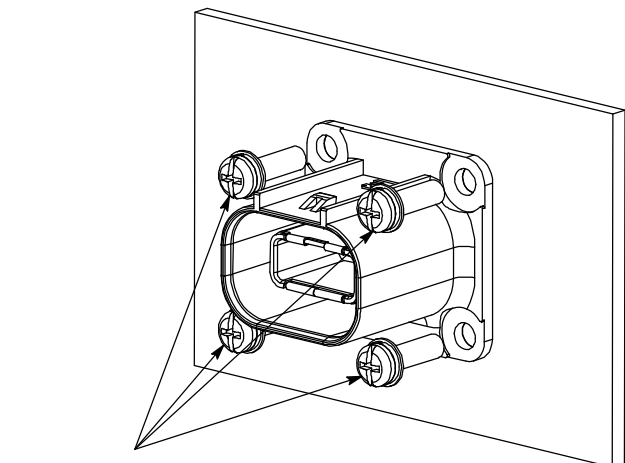
Secure Header with Four M4 Fasteners
