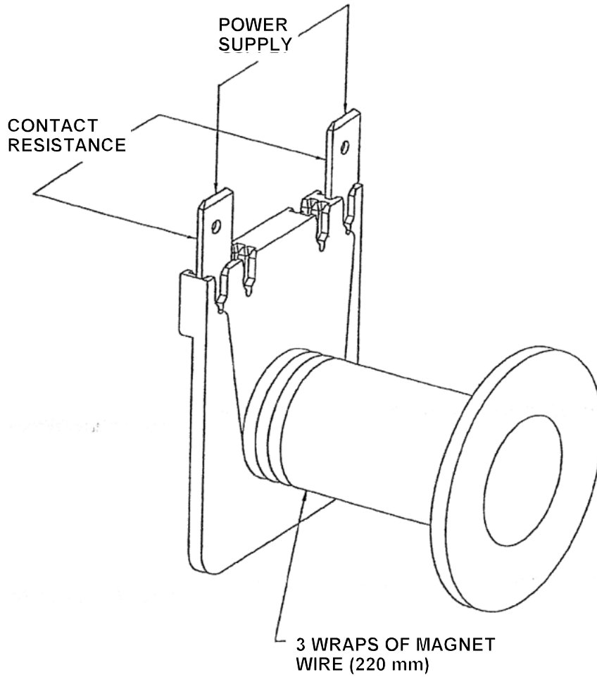
Figure 3 Test Configuration
