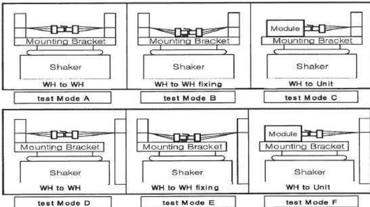
< Fig 5-3 Connector attaching method >
